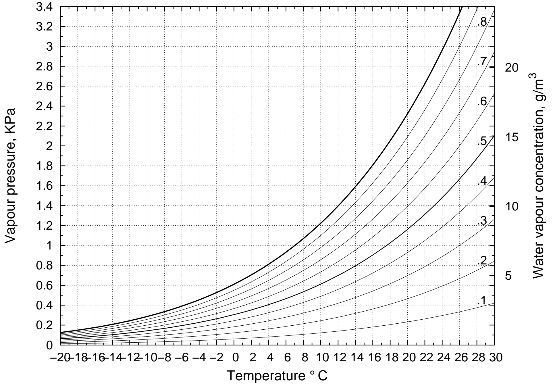
Vapour pressure diagram for water
