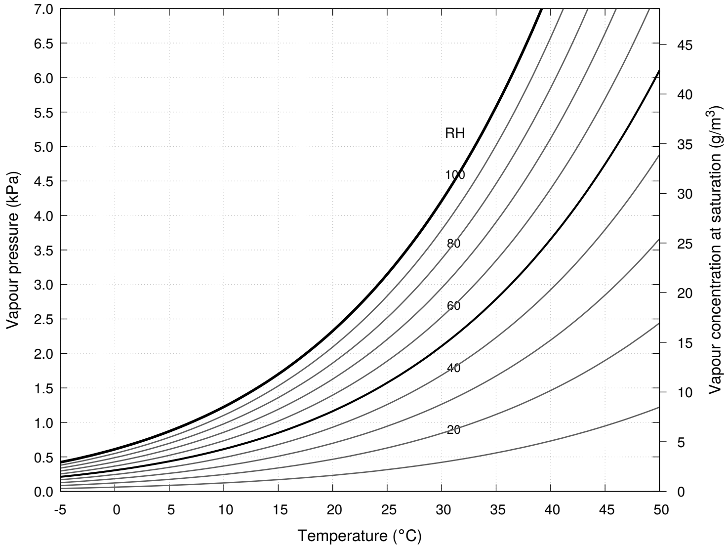
Vapour pressure diagram for water
